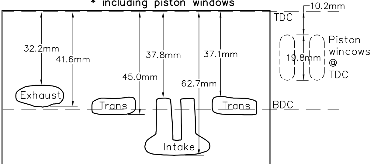
Port Map
